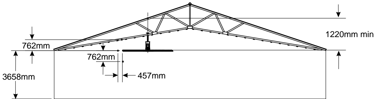
Sloped Roof
